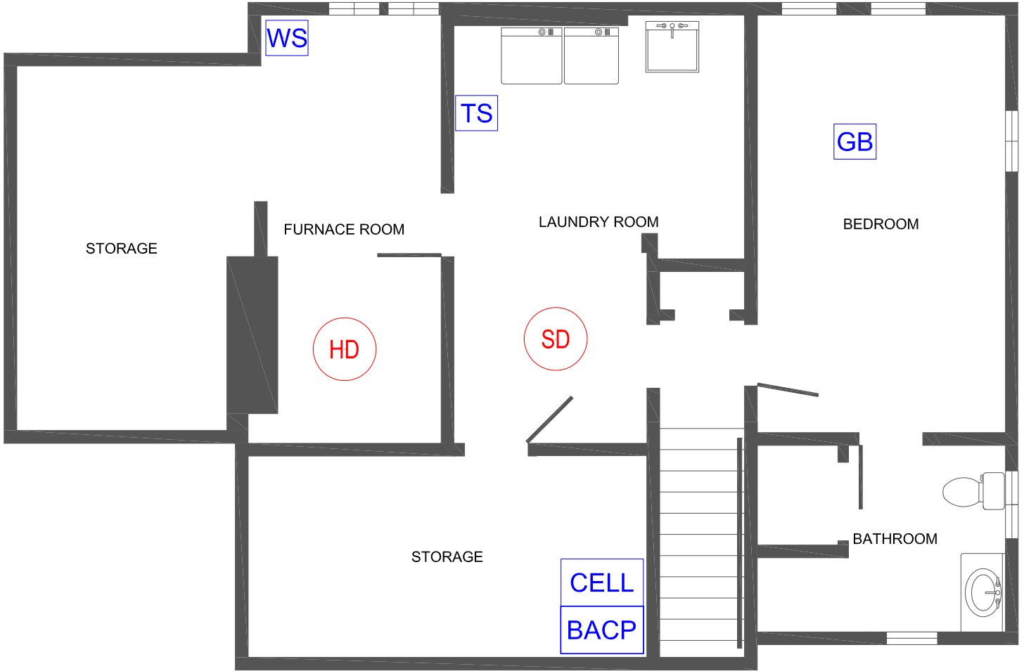
1 BASEMENT FLOOR PLAN SCALE: NTS
